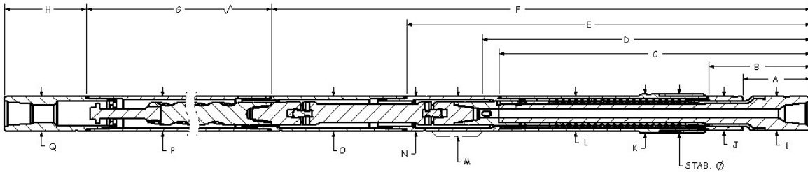
OUTER FISHING DIMENSIONS (FIXED)
